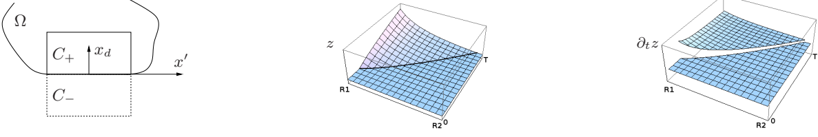
Figure 1: Example for the notation in Section 3.1.3 (left); Graph of the solution z : (0, T) \times (R_1, R_2) \rightarrow \mathbb{R} (middle) and of the time derivative \partial_t z (right).
