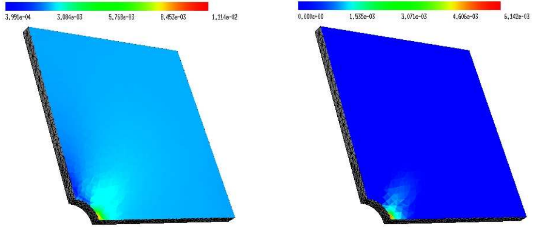
Figure 5: The Frobenius norms of the total strain \varepsilon (left) and of the plastic strain p (right).
